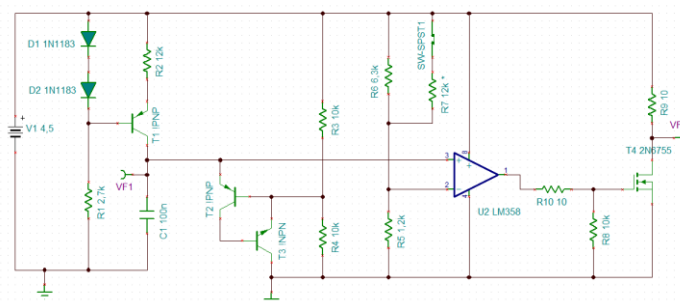
Figure 1. Circuit schematic of the nanoribbons driver.
