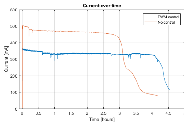
Figure 2. Different control modes and their currents curves.
