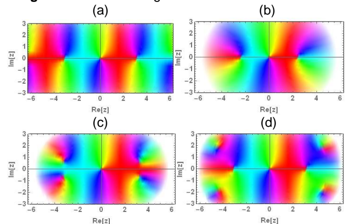
Image 2. Function f(z) by the domain coloring (a), and its Taylor polynomials when (b) (c) and k = 7 (d), around the origin.
