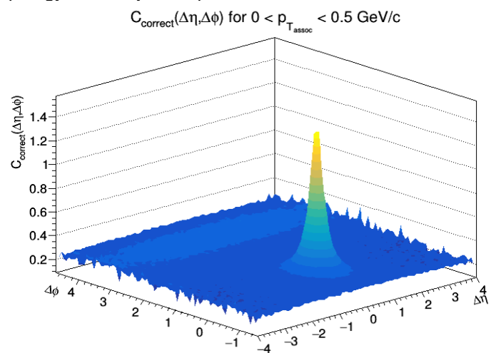
Image 1. C_{correct}(\Delta\eta, \Delta\phi) for 0 < p_{T_{assoc}} < 0.5 GeV. The peak observed at (0,0) is the jet structure.
