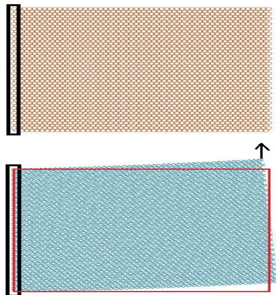
Image 1. Two dimensional structure subjected to external force. On top, original shape and below, deformed shape after application of force. The red box in the second figure indicates the original shape, for comparison
